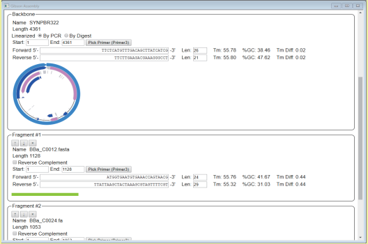
Gibson Assembly
